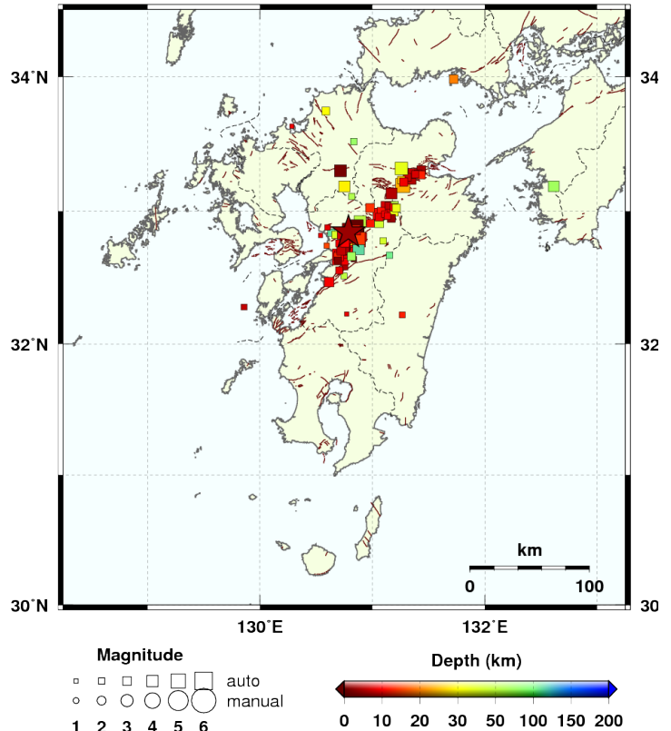
SEVO KYUSHU UNIV. KYUSHU UNIVERSITY Seismicity map in the Kyushu Island 2016/04/15 10:45 - 2016/04/16 10:45 (last 1 day) Last Update (JST): 2016/04/16 10:45 N=314
